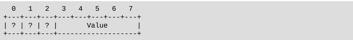
Figure 2: Integer Value Encoded within the Prefix (Shown for N = 5 )
